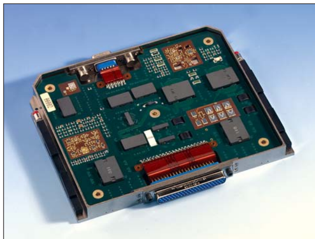
Fig. 1. This 6U COTS dc/dc converter uses COB and planar magnetics technology.
