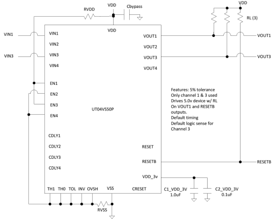
Figure 7. Application example of basic connection
