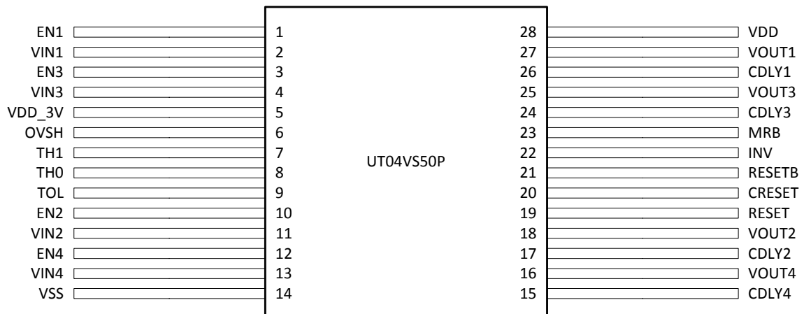
Figure 2. UT04VS50P Pin Configuration
