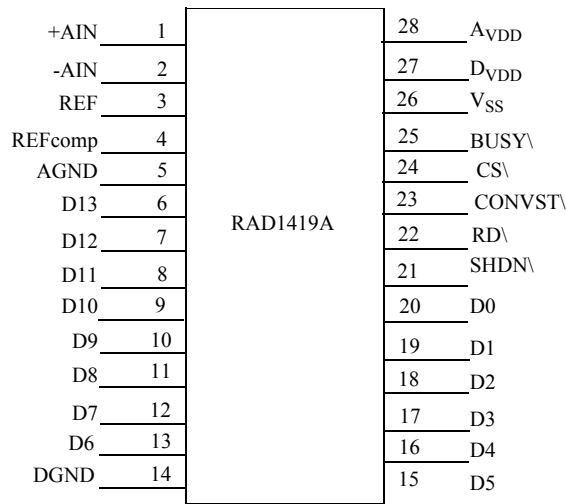
Figure 2. RAD1419A Pinout
