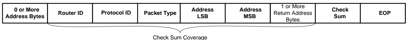
Figure 11. Configuration Port Read Packet Response
