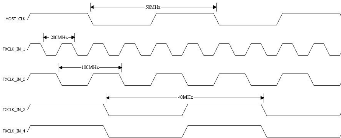
Figure 24. HOST_CLK max TXCLK_IN requirements
