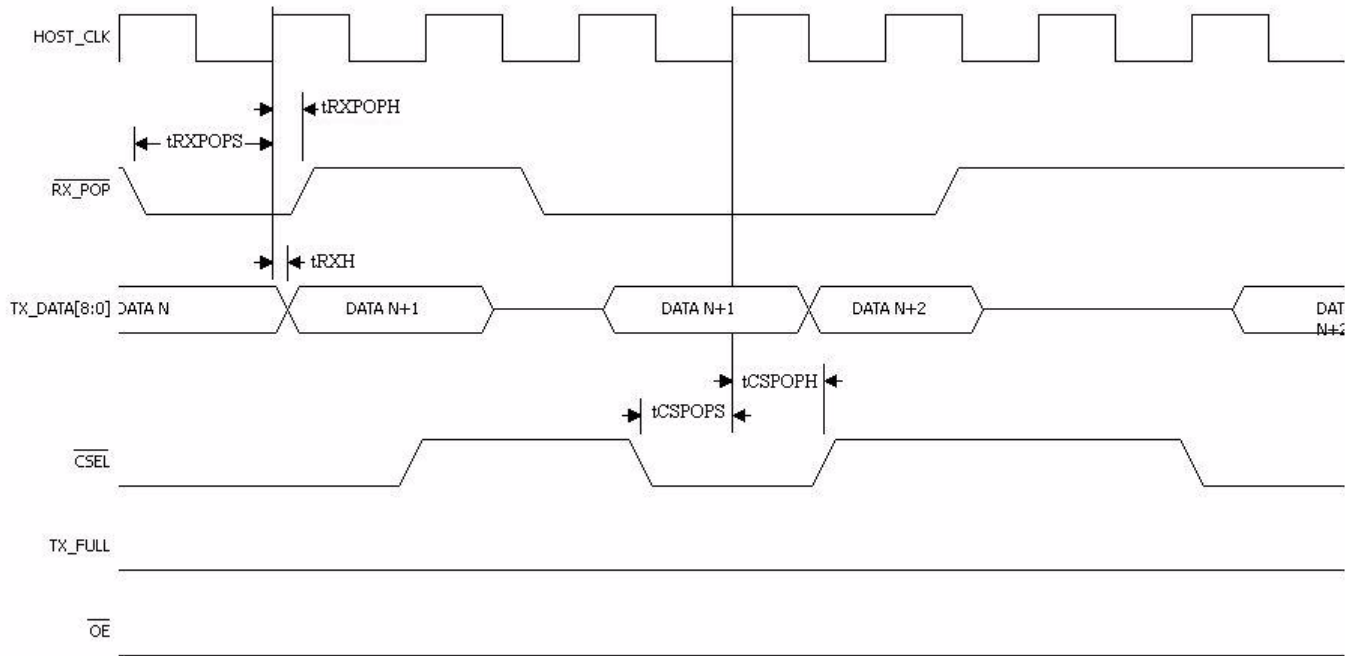
Figure 31. Receive Port POP System port read timing specification, reading data out of System Port FIFO
