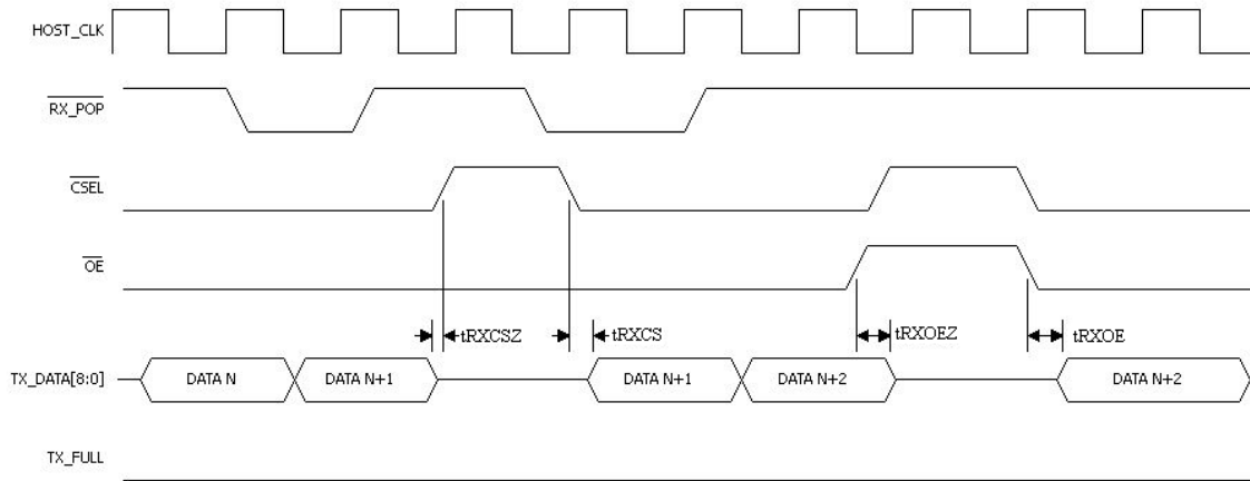
Figure 32. Control Inputs Timing Information
