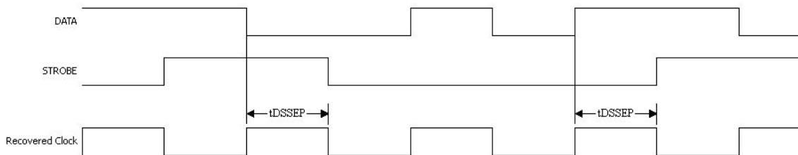
Figure 22. Minimum Data/Strobe Separation LVDS Interface
