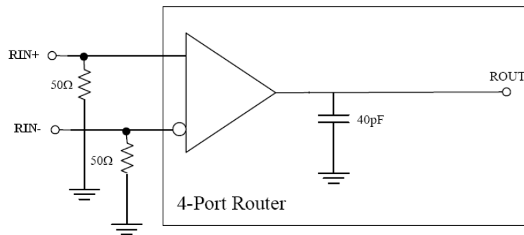
Figure 23. LVDS Receiver Differential Skew, Rise and Fall Time Test Circuit
