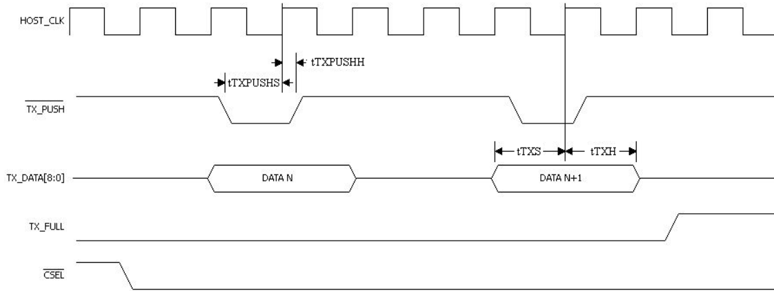
Figure 28. Transmit Port PUSH
