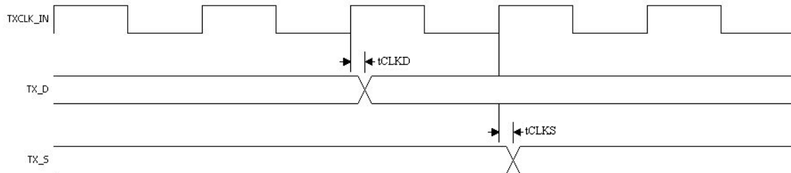
Figure 20. Differential Data Strobe Skew
