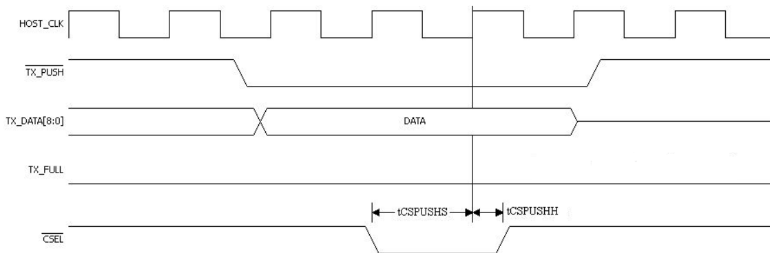
Figure 29. Transmit Port PUSH with Chip Select Transition
