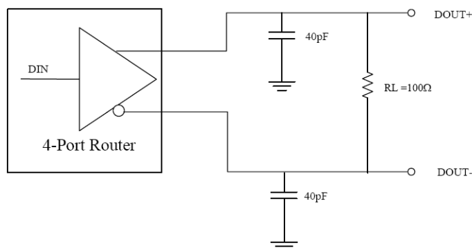
Figure 21. LVDS Driver Differential Skew, Rise and Fall Time Test Circuit
