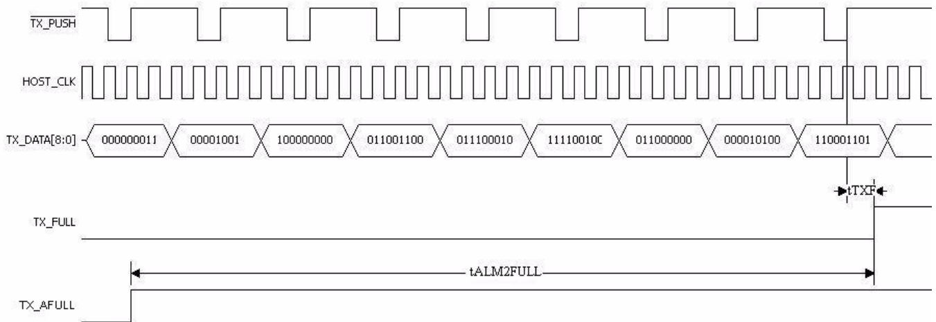
Figure 27. Transmit FIFO Almost Full Flag
